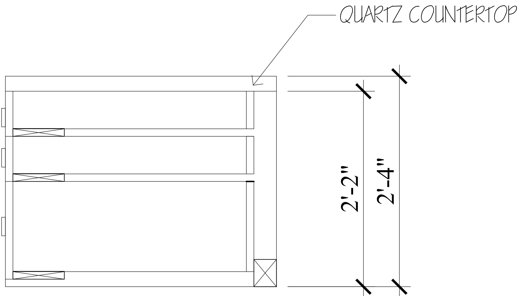
9 RECEPTION DESK SECTION SCALE: 1 1/2" = 1'-0"
