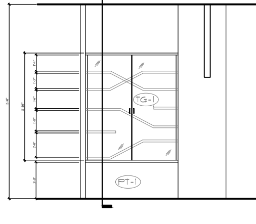
14 SHOWCASE ELEVATION SCALE: 1/4" = 1'-0"
