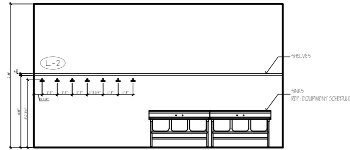
10 ANTI ROOM ELEVATION SCALE: 1/4" = 1'-0"
