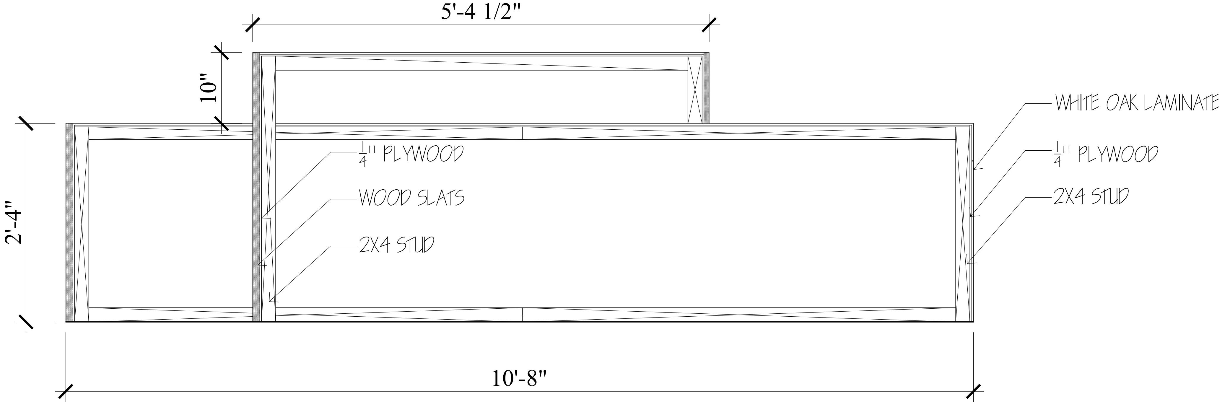
8 SHOWCASE SECTION SCALE: 1 1/2" = 1'-0"
