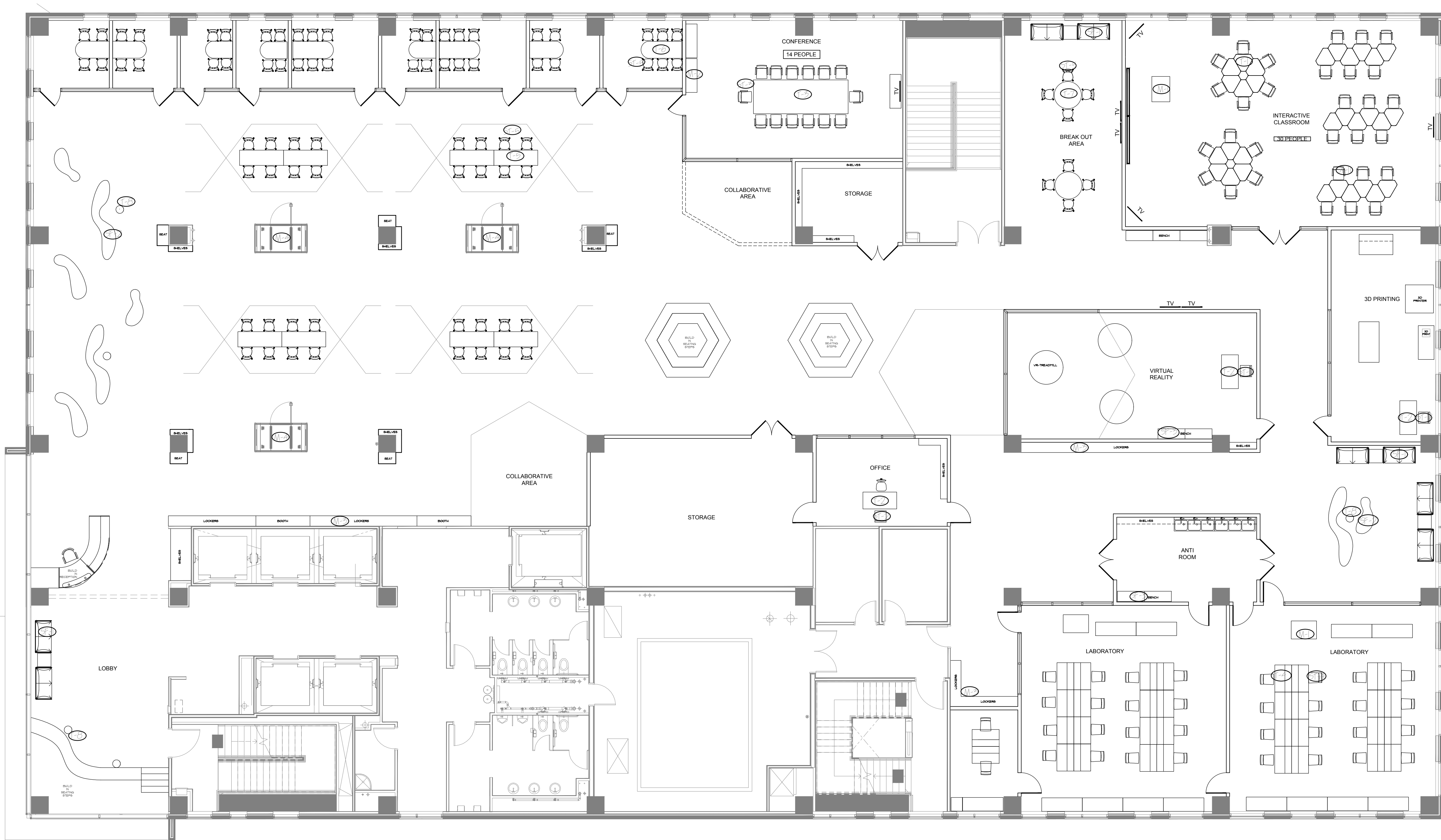
1 FURNITURE FLOOR PLAN SCALE: 1/8" = 1'-0"
