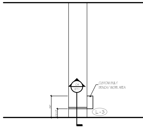
5 COLUMN ELEVATION SCALE: 1/4" = 1'-0"
