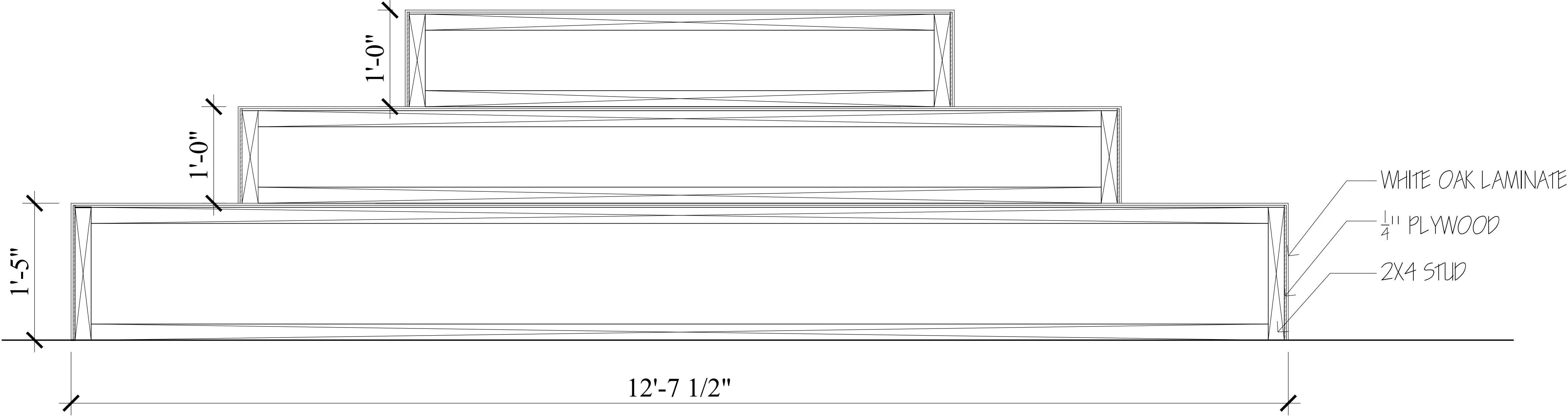
7 HEXAGON BENCH SECTION SCALE: 1 1/2" = 1'-0"
