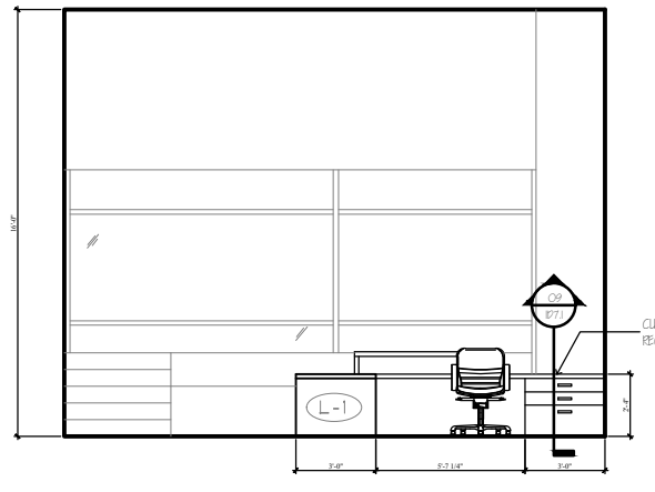
13 RECEPTION ELEVATION SCALE: 1/4" = 1'-0"
