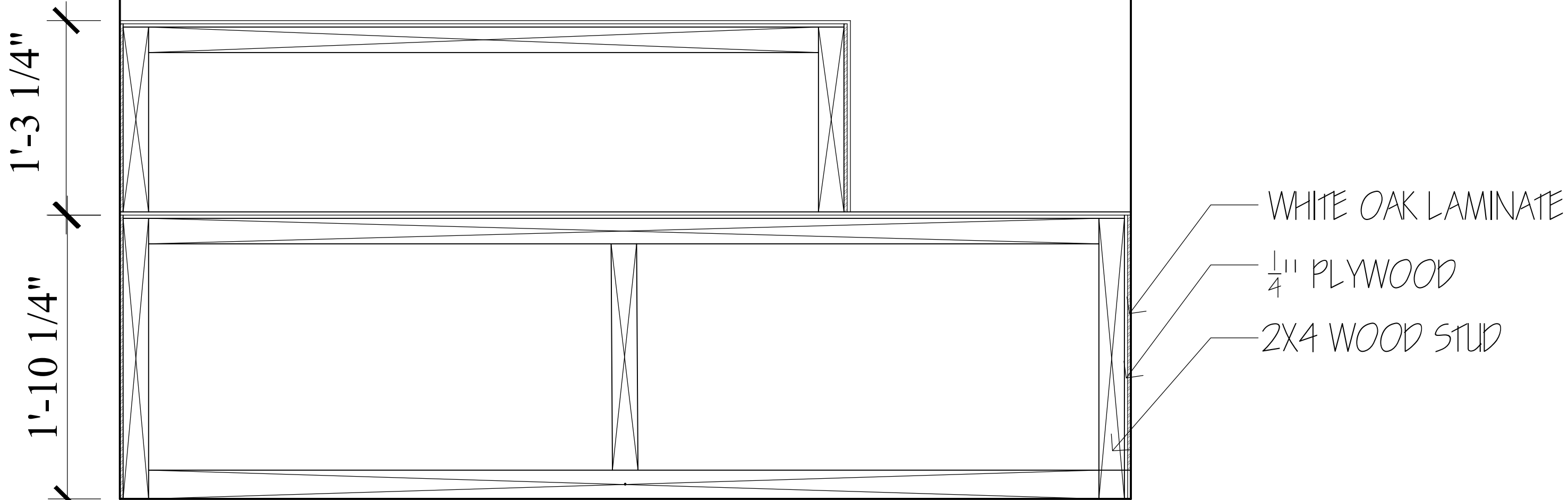
1 LOBBY STAIR SECTION SCALE: 1/2" = 1'-0"
