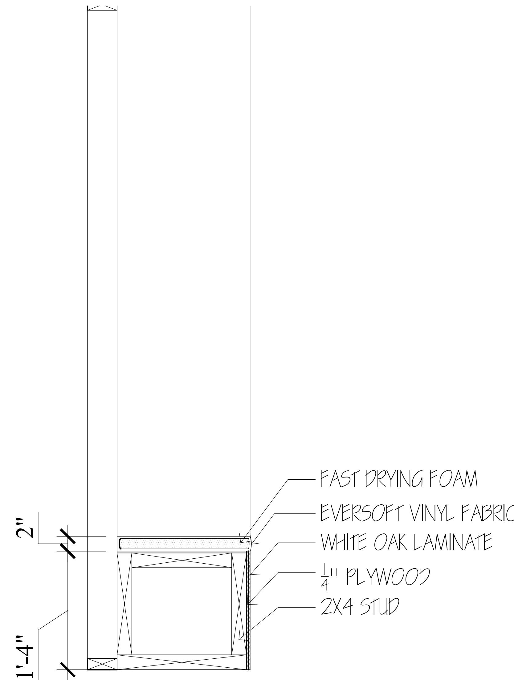
5 BENCH SECTION SCALE: 1/2" = 1'-0"
