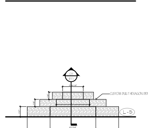
9 HEXAGON BENCH ELEVATION SCALE: 1/4" = 1'-0"
