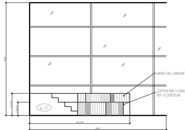
3 WEST STAIR ELEVATIONS SCALE: 1/4" = 1'-0"
