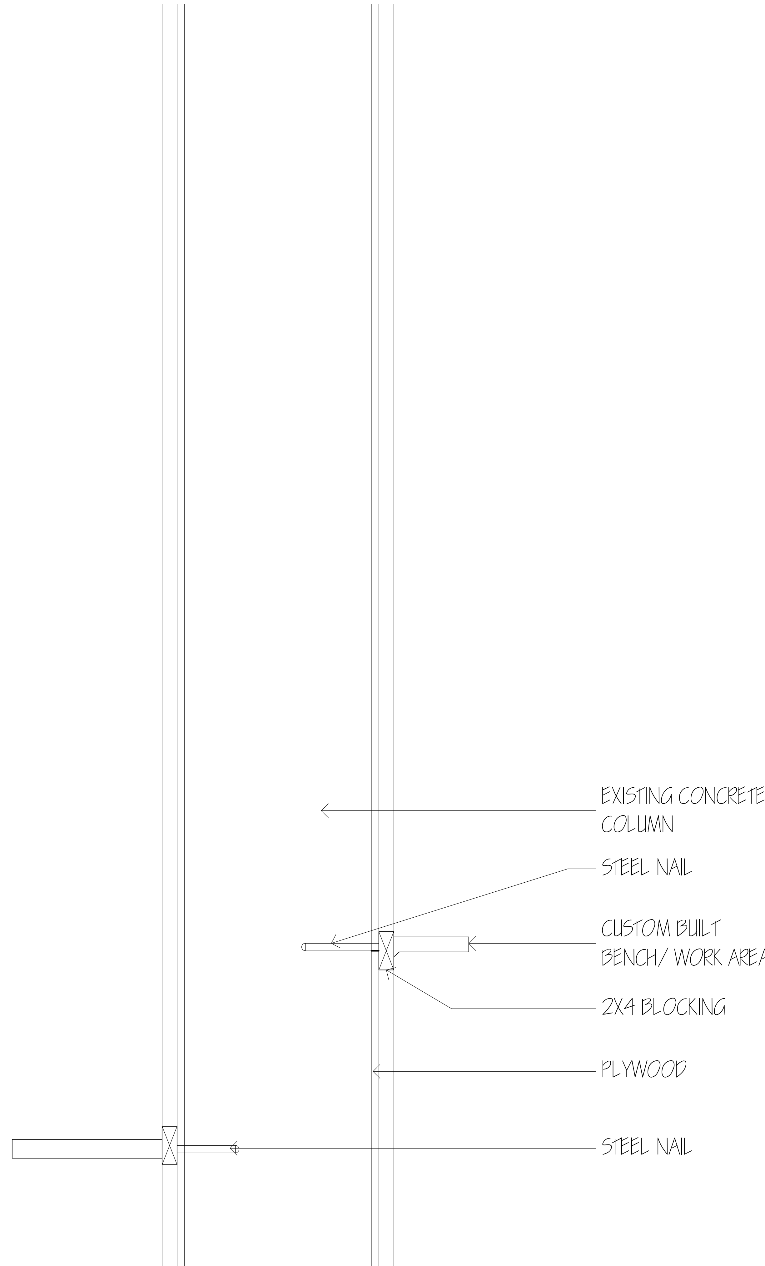
4 COLUMN BENCH SECTION SCALE: 1/2" = 1'-0"
