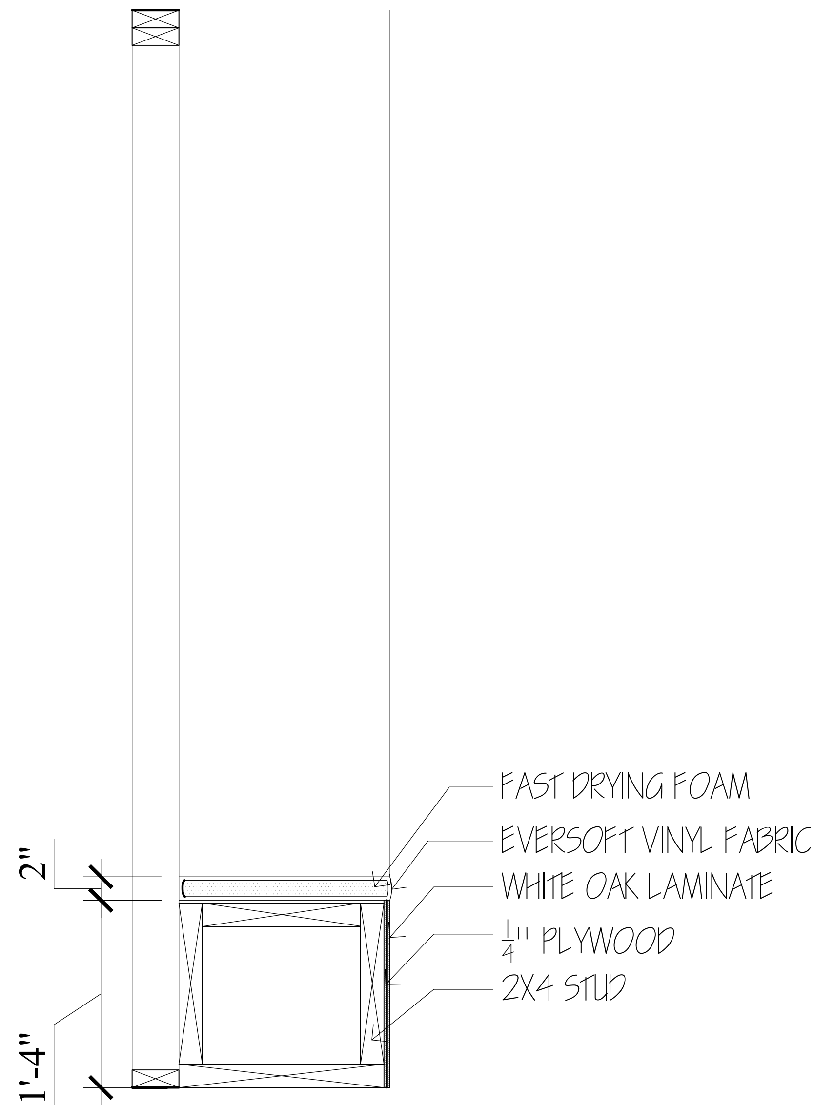
3 LOCKER BENCH SECTION SCALE: 1/2" = 1'-0"
