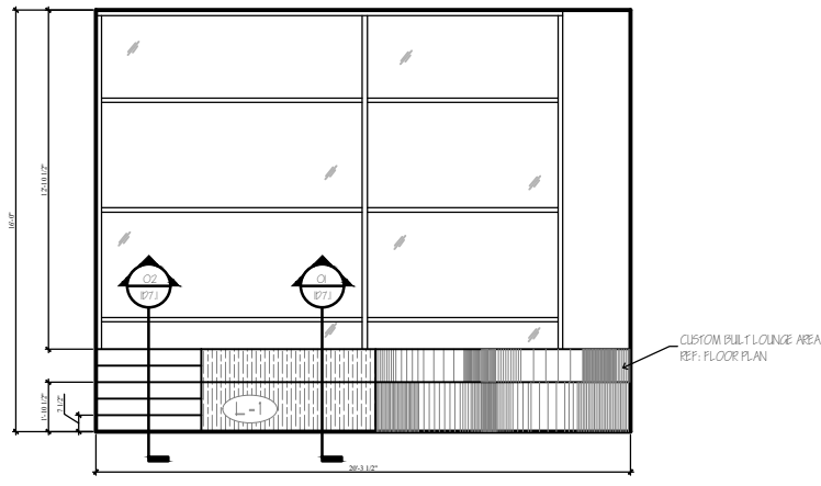
2 SOUTH STAIR ELEVATION SCALE: 1/4" = 1'-0"
